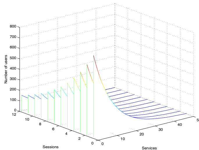
Figure 2. A simulated Web site with 50 services and 12 sessions is represented. An exponential decrease of the number of users with respect to the logged-in sessions and the clicked services is shown.
