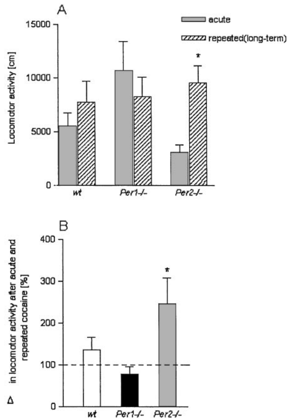
Fig. 3. Long-term sensitization in Per mutants. Locomotor responses to acute and repeated saline/cocaine injections in wild-type (wt) mice or mice carrying a mutation in mPer1 and mPer2 genes after a withdrawal period of 3 weeks are shown. (A) Mean locomotor activity \pm SEM after acute and repeated cocaine injections. Two-way ANOVA revealed that cocaine sensitization differed significantly for the different genotypes (see text). Further statistical comparison between acute and repeated (long-term) treatment for each genotype showed the following differences: wt, P = 0.37 ; Per1 mutant, P = 0.44 ; and Per2 mutant, P = 0.007 . * indicates a significant difference to acute cocaine P < 0.01 . (B) The increase in locomotor activity after repeated cocaine injections was also calculated as percentage difference in activity to acute cocaine injection. One-way ANOVA revealed a genotype effect [ F(2,16) = 7.15 , P = 0.007 ]. * indicates a significant difference to wt mice, P < 0.05 .
